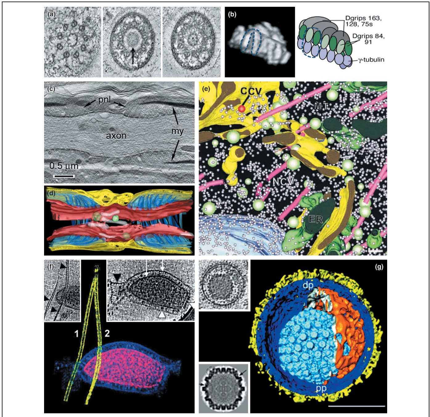
Figure 2. Tomograms and 3D models of biological structures. (a) Slices (each \sim 1.5 -nm thick) from a tomogram of a basal body from Chlamydomonas reinhardtii . The two-layered arrangement of the material in the ninefold star is apparent from the middle slice, which lacks the star (arrow). Images reproduced, with permission, from Ref. [6]. (b) A 3D reconstruction of the \gamma -tubulin ring complex, viewed as shaded surfaces identified by a grayscale threshold (left) and as a model (right) in which the molecular components are identified. Images reproduced, with permission, from Ref. [7]. (c) Slice from a tomogram of a node of Ranvier, showing the axon, the myelin sheath (my) and the paranodal loops (pnl). Scale bar = 0.5 \mu m. (d) Features of the node of Ranvier shown in a 3D model based on many tomographic slices such as those shown in (c). The volume comprises a thickness of approximately 1.5 \mu m and an area of approximately 2 \times 5 \mu m. The axolemma (red), paranodal loops (blue), mitochondria (white) and intra-axonal vesicles (green) are indicated. Images in (c,d) reproduced, with permission, from Ref. [9]. (e) Model constructed from hand-drawn contours marking the boundaries of cellular components in a tomogram of the phragmoplast formed during pollen development in Arabidopsis thaliana . Scale bar = 50 nm. Image reproduced, with permission, from Ref. [11]. (f) Images of the archaeon Pyrodicticum . The cell and its associated extracellular fibers, called cannulae (small black arrowheads), are visible in the two tomographic slices (top left and right). The plasma membrane and the S-layer can be seen clearly (white arrows) and there are particles in the periplasmic space (white arrowhead). At one end of the cell, the S-layer bulges (large black arrowhead). The pseudocolored representation shows the cannulae in yellow (labeled 1 and 2), the cytoplasm in magenta, and the periplasm and S-layer in blue. Images reproduced, with permission, from Ref. [49]. (g) The virion of Herpes simplex virus. Top inset, a 5.2-nm slice from a tomogram showing the envelope (blue and yellow), the protein-containing 'tegument' (orange) within it, and the nucleocapsid (light blue). Bottom inset, results of averaging to improve the image signal-to-noise ratio. Tomography also reveals the pleiomorphic structures surrounding the nucleocapsid, although the signal-to-noise ratio is lower. The pseudocolored representation shows a model of the whole virus based on cryo-ET. Scale bar = 100 nm. Images reproduced, with permission, from Ref. [58]. Abbreviations: CCV, clathrin-coated vesicle; CP, cell plate; dp, distal pole; ER, endoplasmic reticulum; MT, microtubule; NCV, non-coated vesicle; pp, proximal pole.
